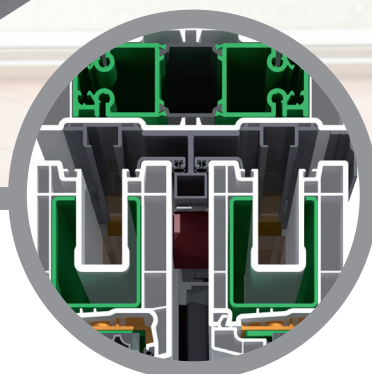
Hebeschiebetür beide Flügel parallel verschiebbar Lift and slide door both casements parallel slidable
